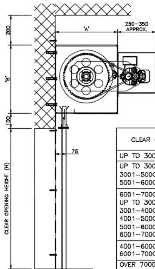
SECTION VIEW
